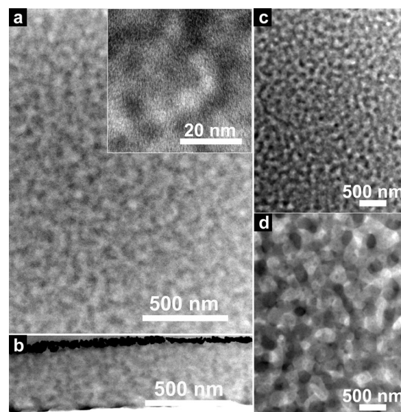
Figure 1. Plan-view TEM images of 1:1 (by weight) blends of PS/P(S- r -2VP)56k with PS having an M of 26k (a), 34k (c), and 55k (d). The images show co-continuous nanostructures with molecular-weight-dependent sizes. b) A cross-sectional TEM image of the same sample as shown in a) confirms that the co-continuous structure spans the film thickness. In all images, P(S- r -2VP)-rich phases appear darker because of staining with \text{I}_2 vapor.
