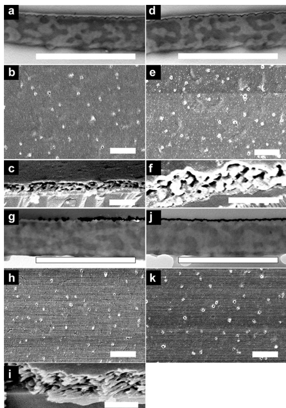
Figure 4. Blend films of 1:1 (by weight) PS26k/P(S- r -2VP)56k prepared on a silicon wafer (a–c), a gold-coated silicon wafer (d–f), a mica substrate (g–i), and a polyimide substrate (j–l). Cross-sectional TEM images (a, d, g and j), and top-view (b, e, h and k) and cross-sectional (c, f and i) SEM images after selective solvent extraction of P(S- r -2VP)-rich domains. Similar co-continuous structures are observed, regardless of the substrate type (scale bars: 1 \mu m).
